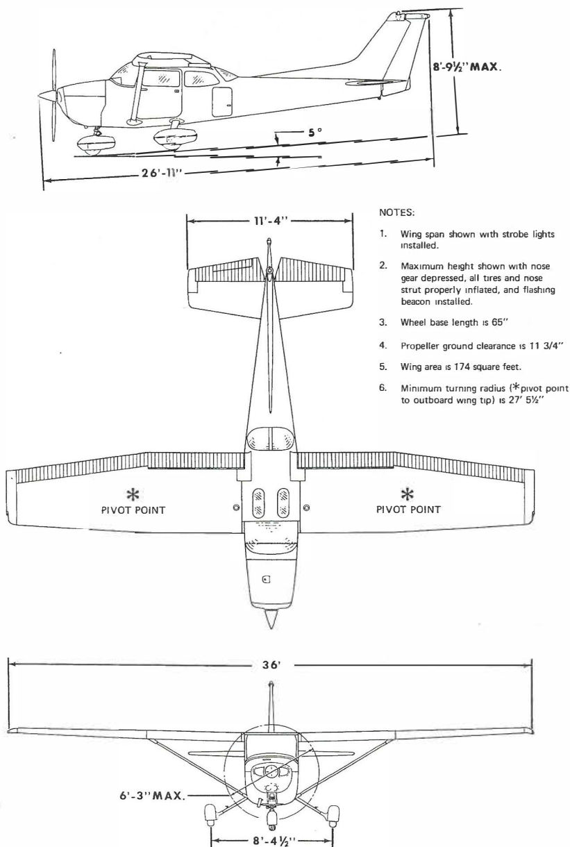
Figure 1-1. Three View
