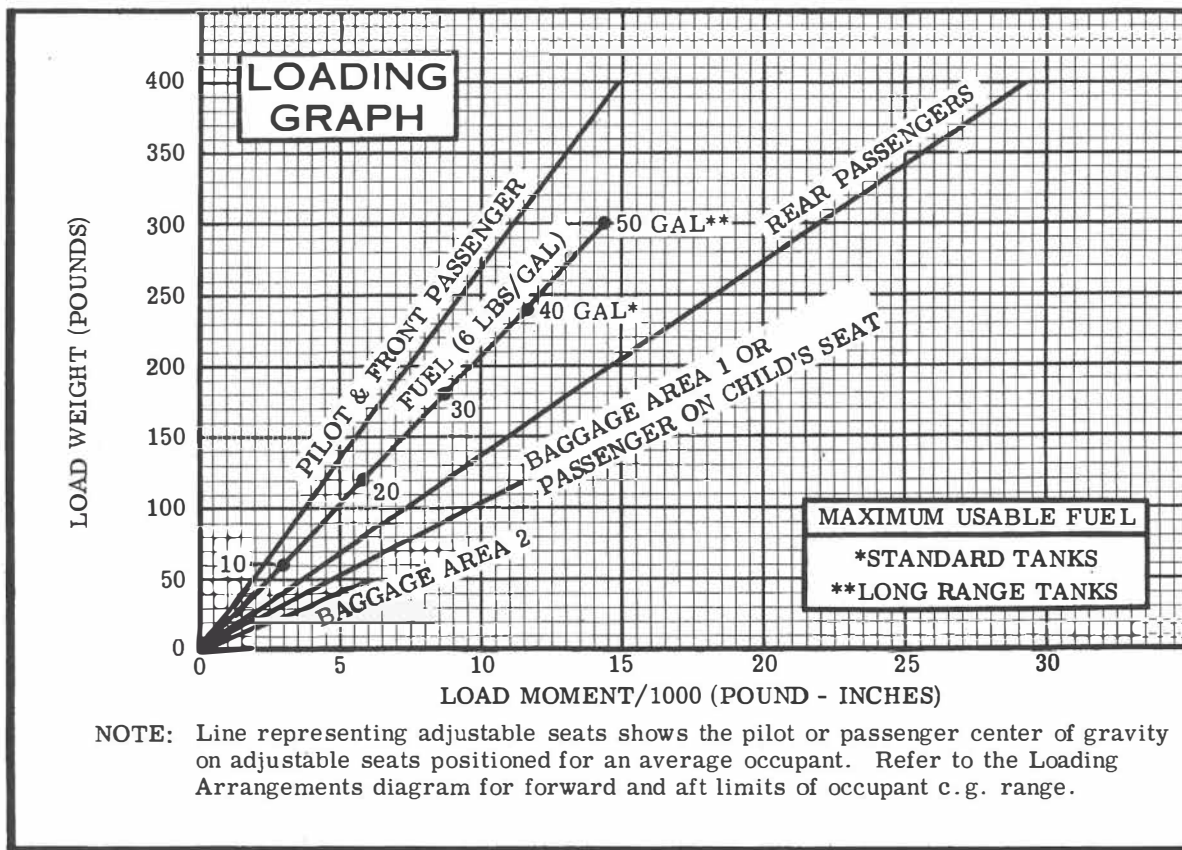
Figure 6-6. Loading Graph
